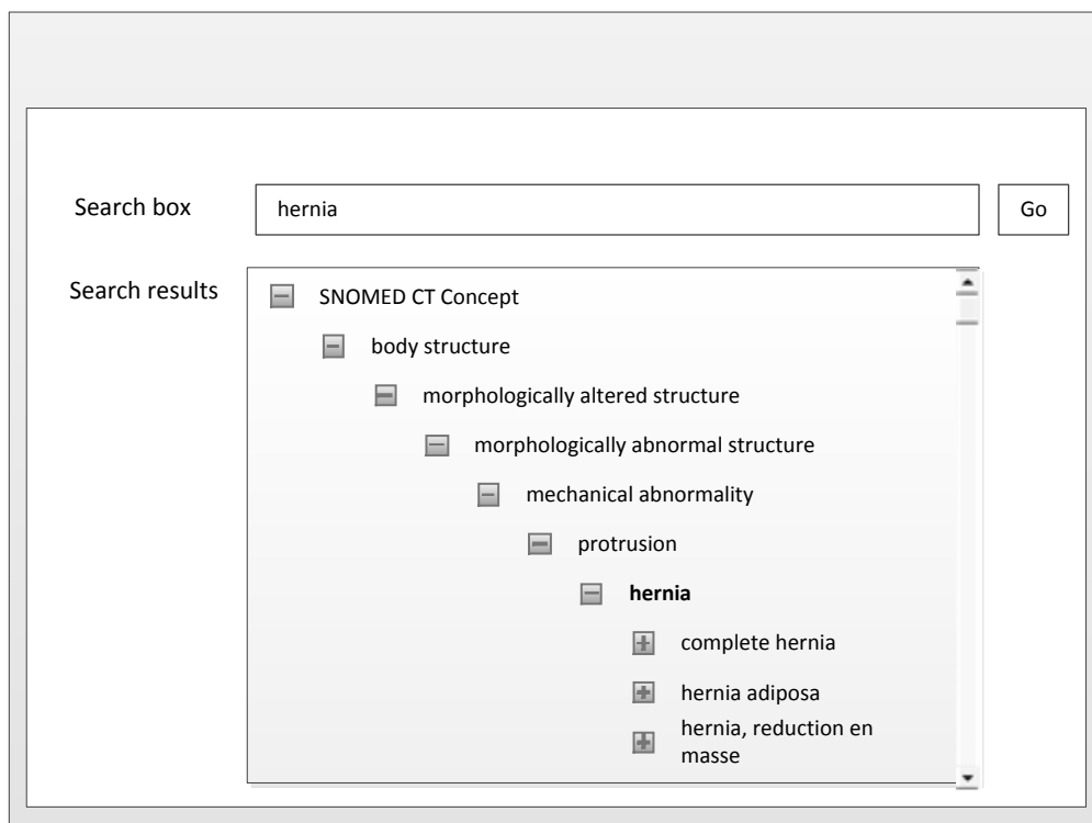
Figure 27 The subtype hierarchy
