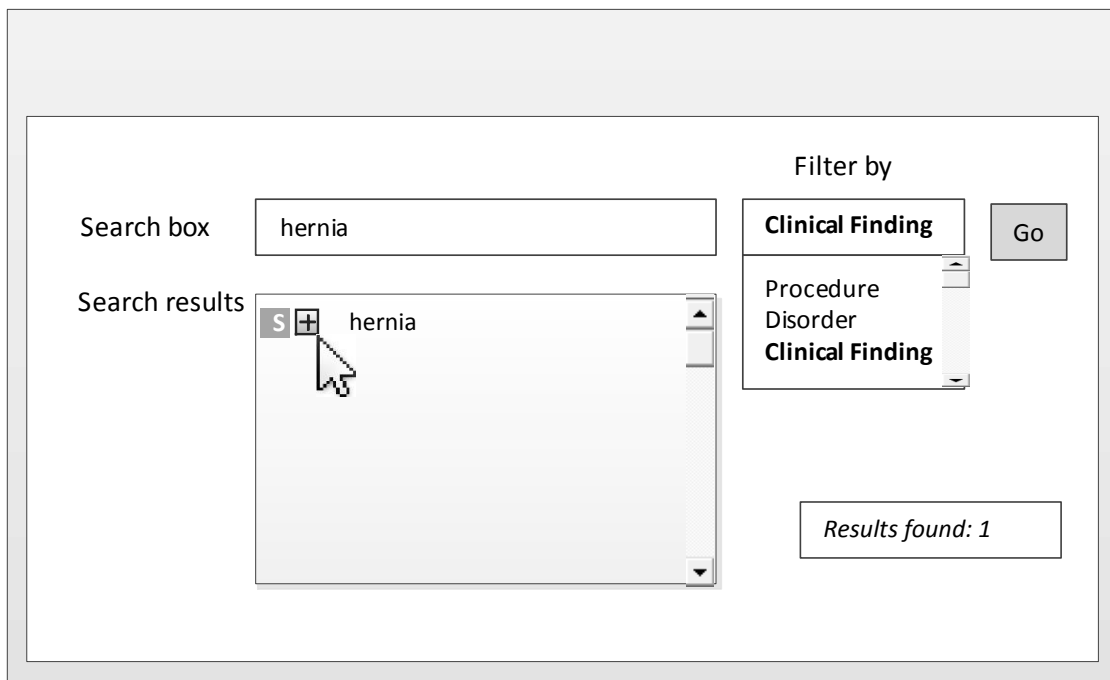
Figure 26 Subsumed Concepts nested under "hernia"
