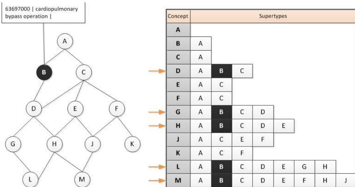
Figure 40 Using transitive closure to constrain data entry according to supertype relevance
