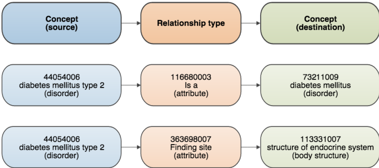
Example of attribute relationships
