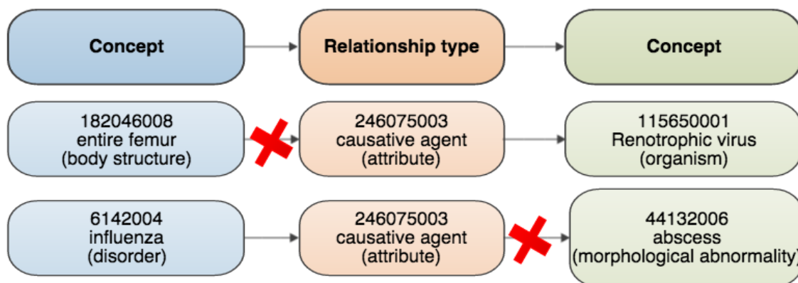
Example of erroneous relationships
