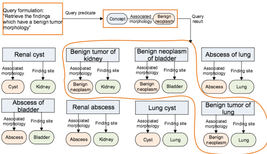
Example: Result of retrieving concepts with |associated morphology| specified as |benign neoplasm|
