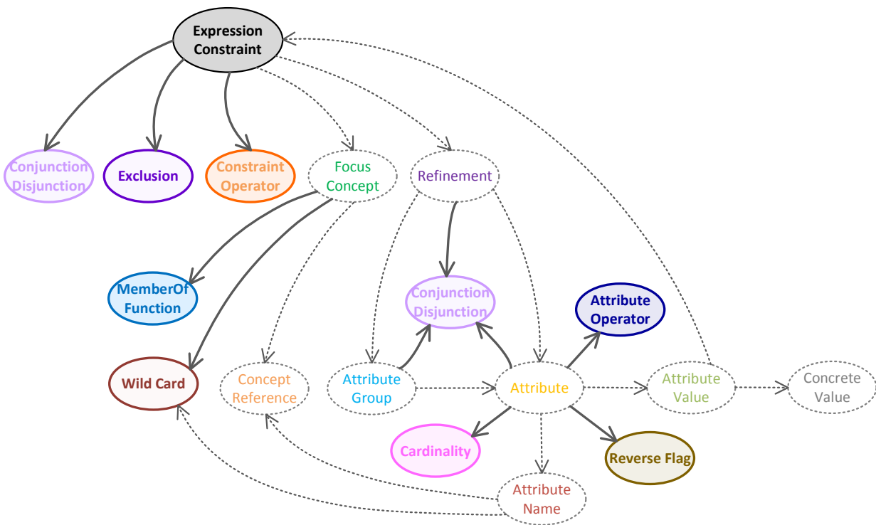
Figure 1: Abstract Model of an Expression Constraint
