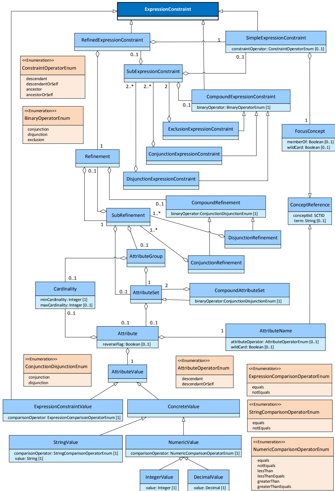
Figure 3: Logical Model of Expression Constraint Language
