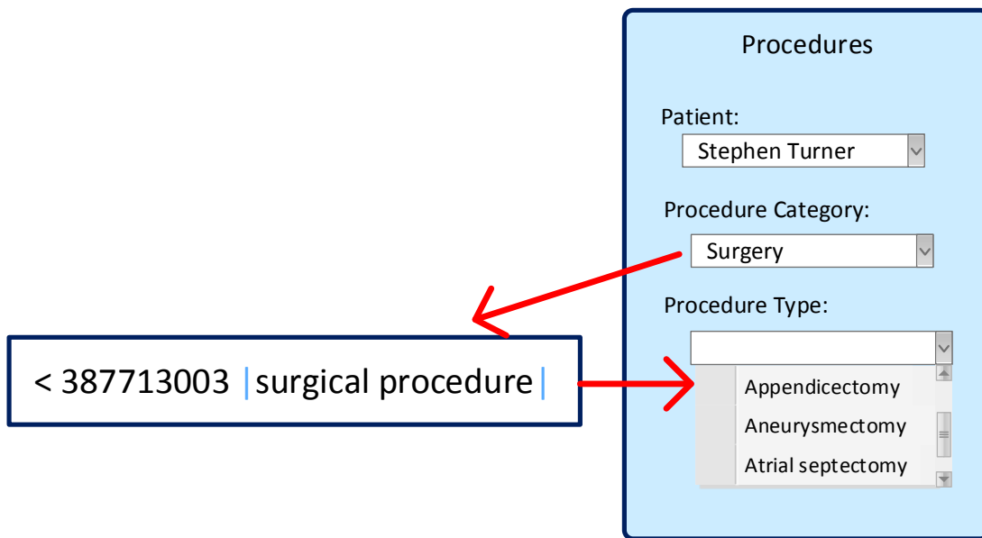
Figure 4: Authoring using expression constraint templates
