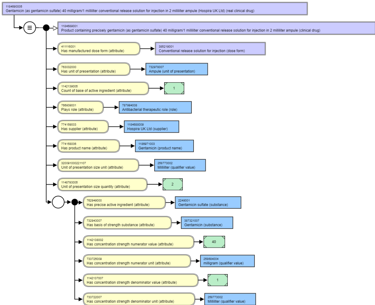
Figure 33: Single active ingredient substance (concentration and presentation strength) with equivalent clinical drug real clinical example inferred view
