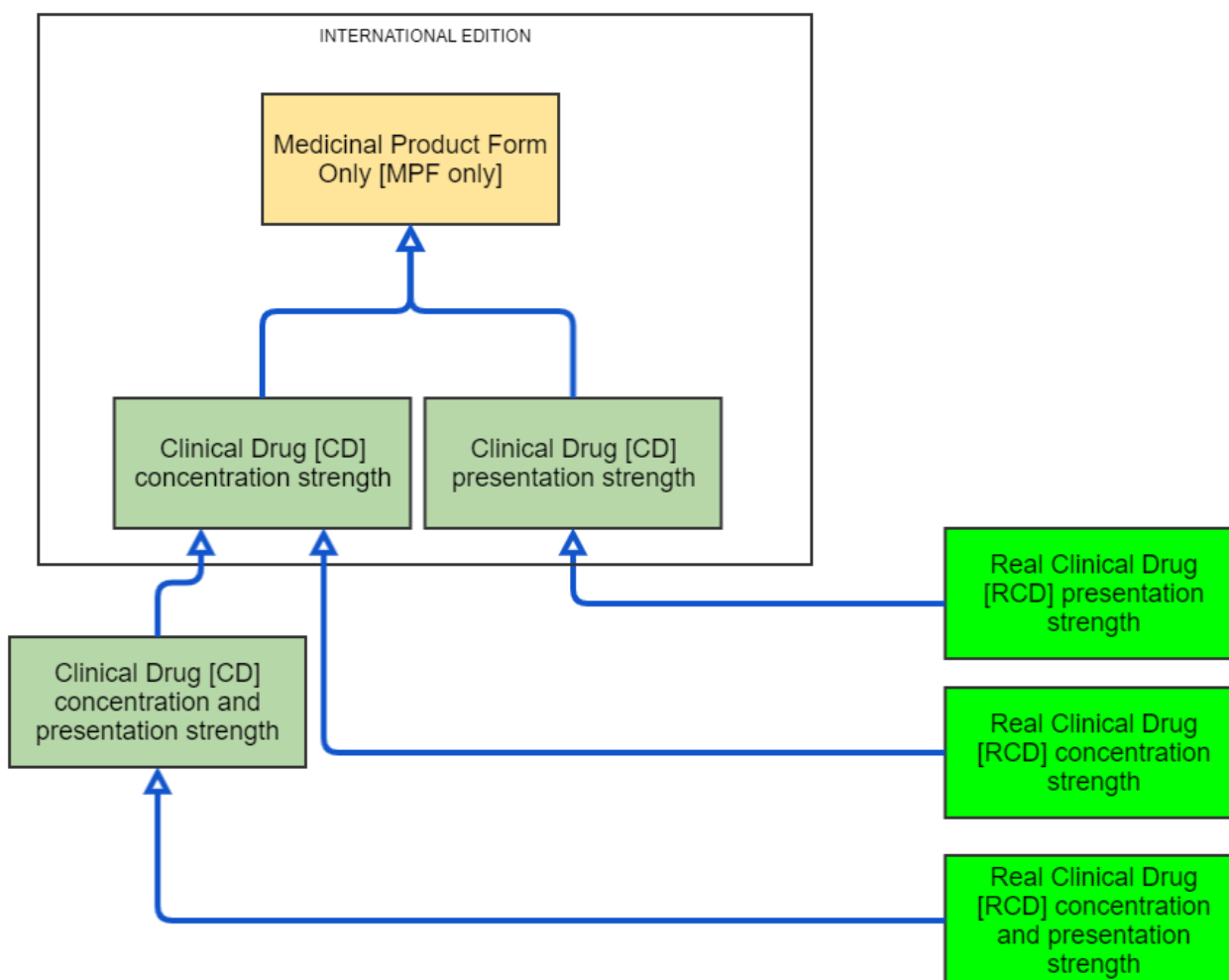
Figure 21: Diagram of relationships and optionality for presentation strength and concentration strength Clinical Drug and Real Clinical Drug
