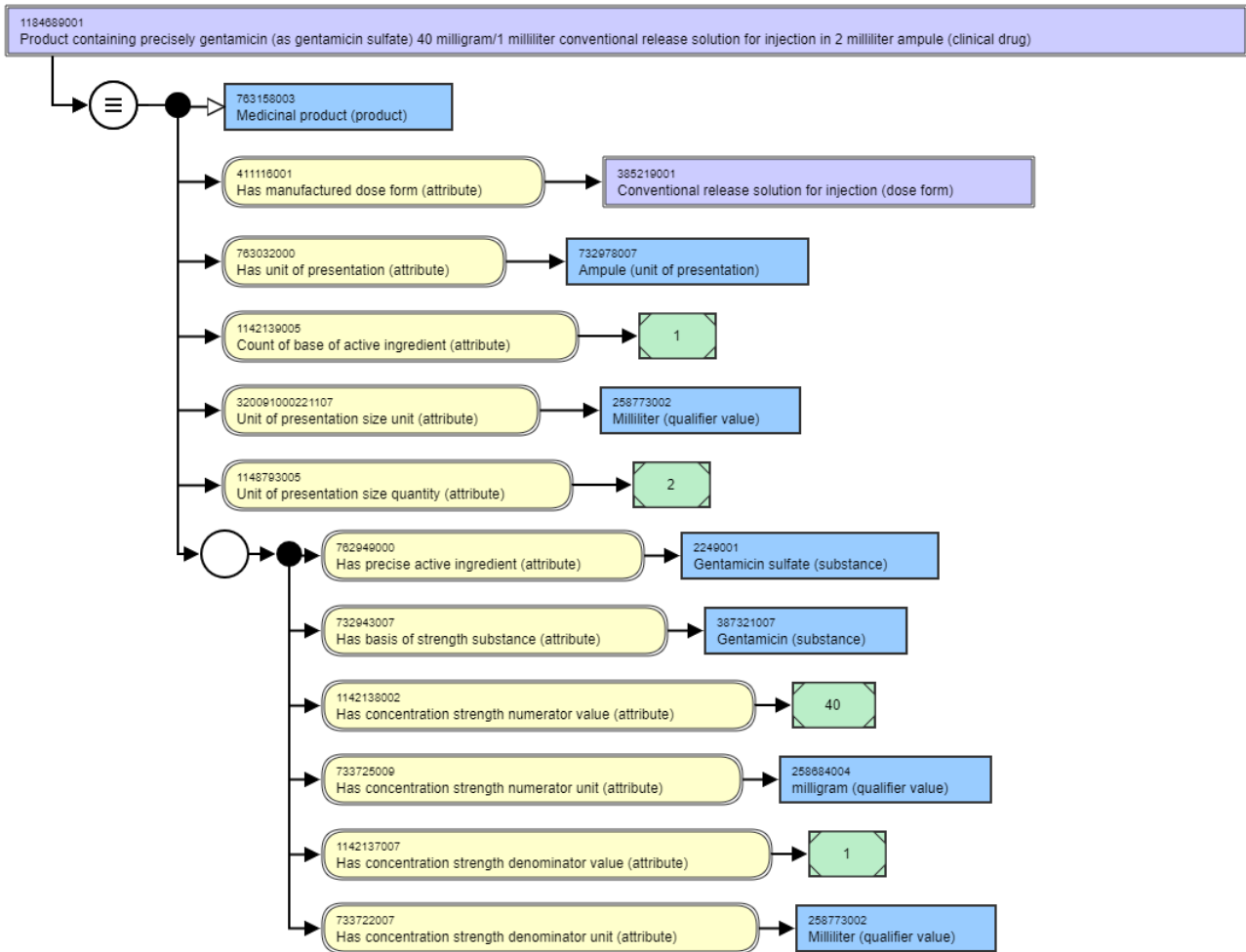
Figure 19: Clinical drug (CD) concentration and presentation strength for a national extension stated view
