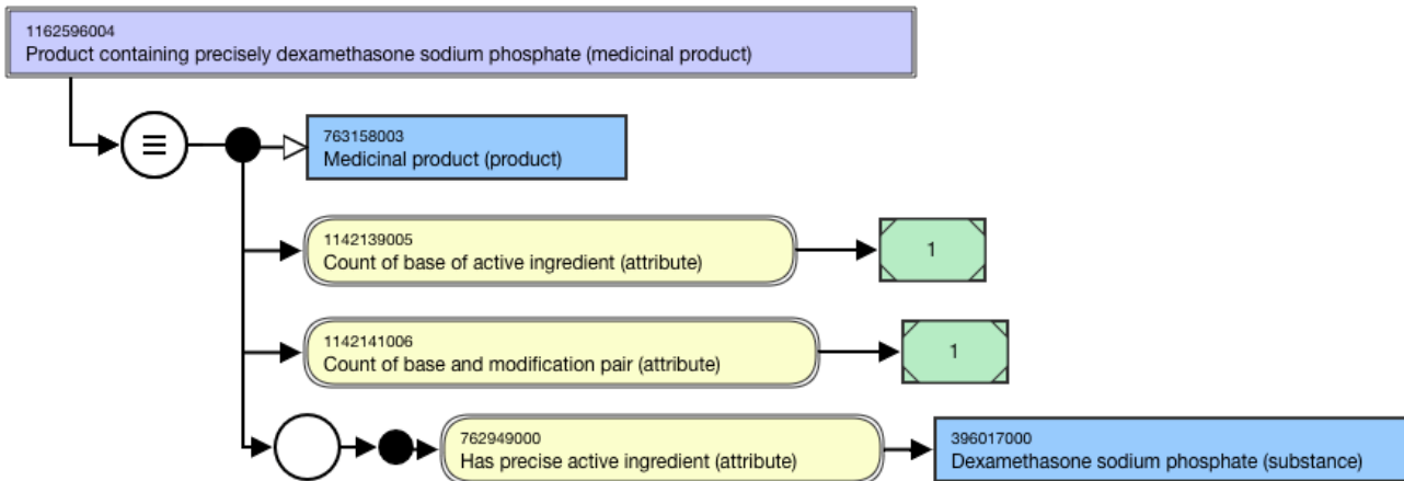
Figure 13: Single Ingredient Medicinal Product (precisely) example stated view
