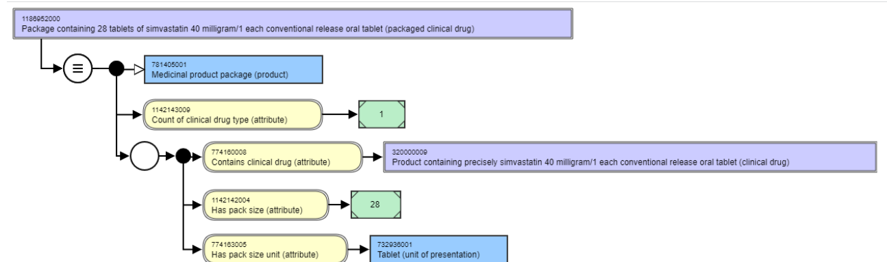
Figure 38: Example of a presentation strength packaged clinical drug - stated view
