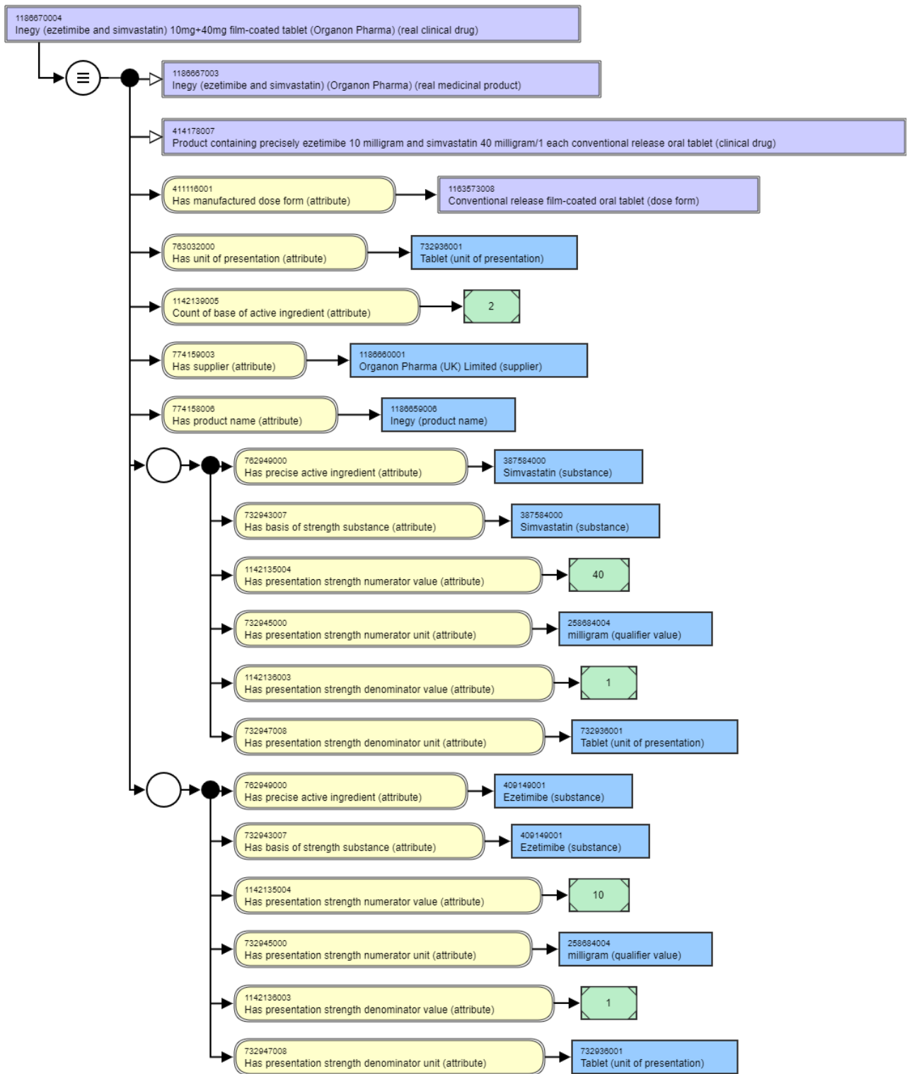
Figure 29: Multiple active ingredient substance (presentation strength) real clinical example inferred view
